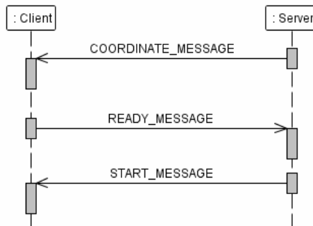
Figure 5- Starting game in two-player mode scenario
