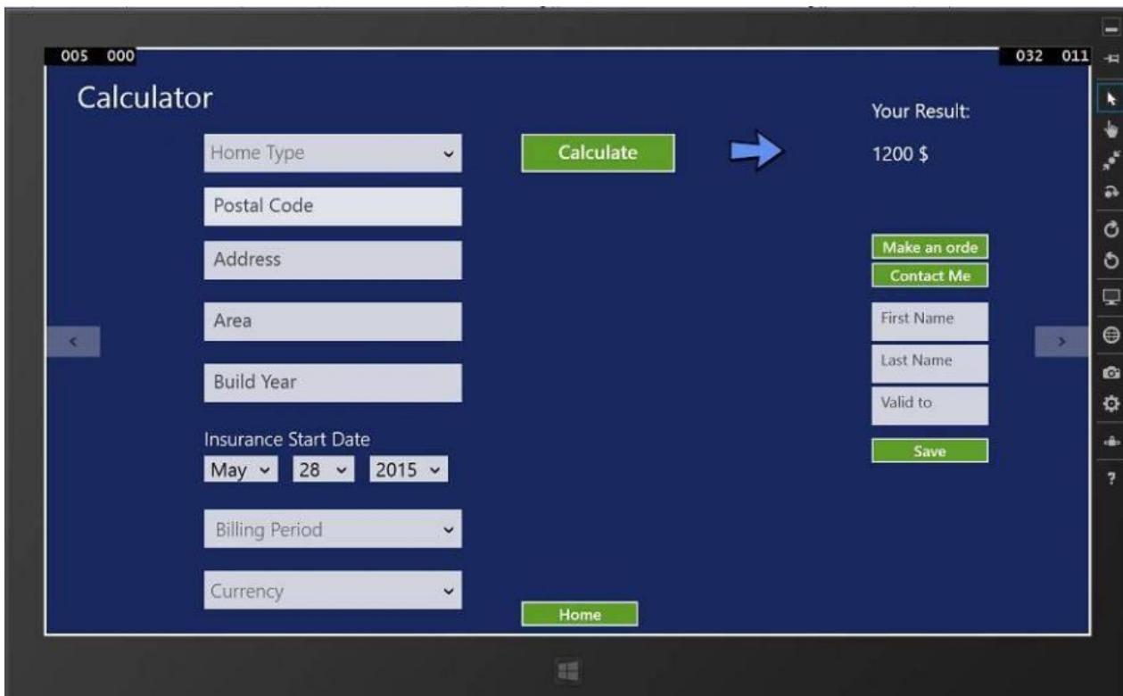
Fig 3. Calculator GUI
