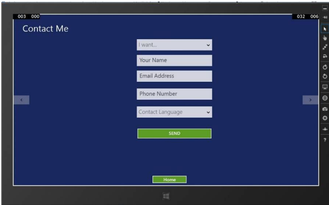
Fig 4. Contact GUI
