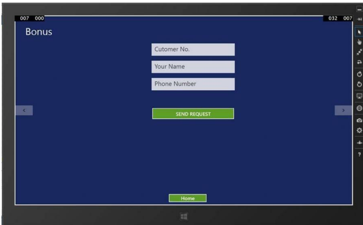
Fig 5. Bonus GUI
