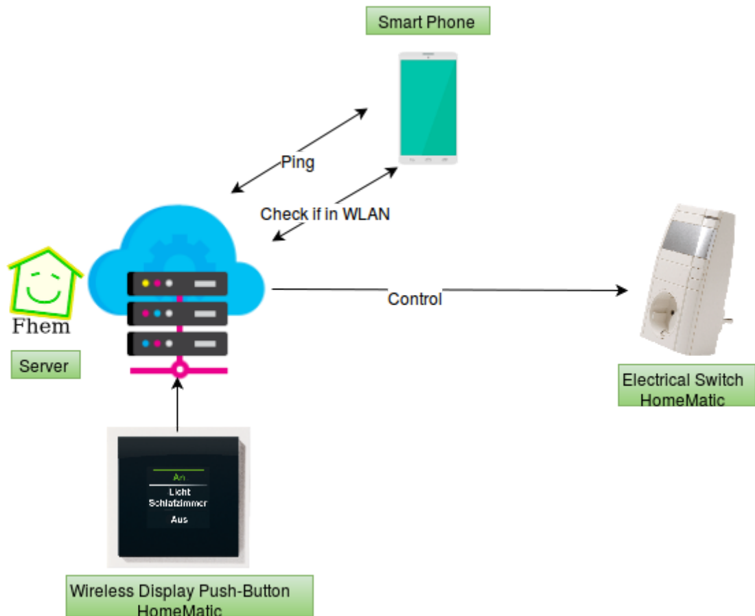
Figure 1. Data Flow Architecture in The Solution
